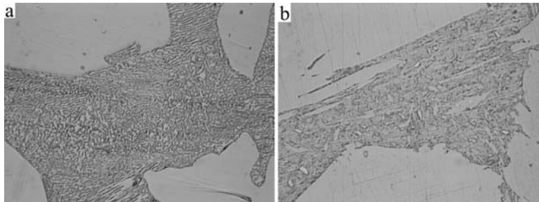
Fig. 2 Optical micrographs (500 \times ) obtained for the annealed samples: a – Cu–10 mass%Al alloy; b – Cu–10 mass%Al–4 mass%Ag alloy
